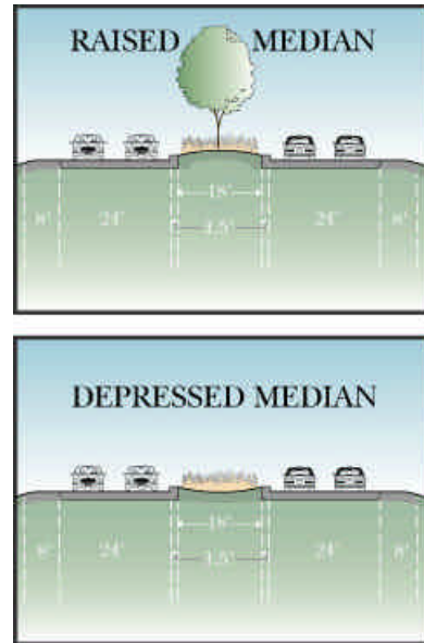
Details of Median Design
